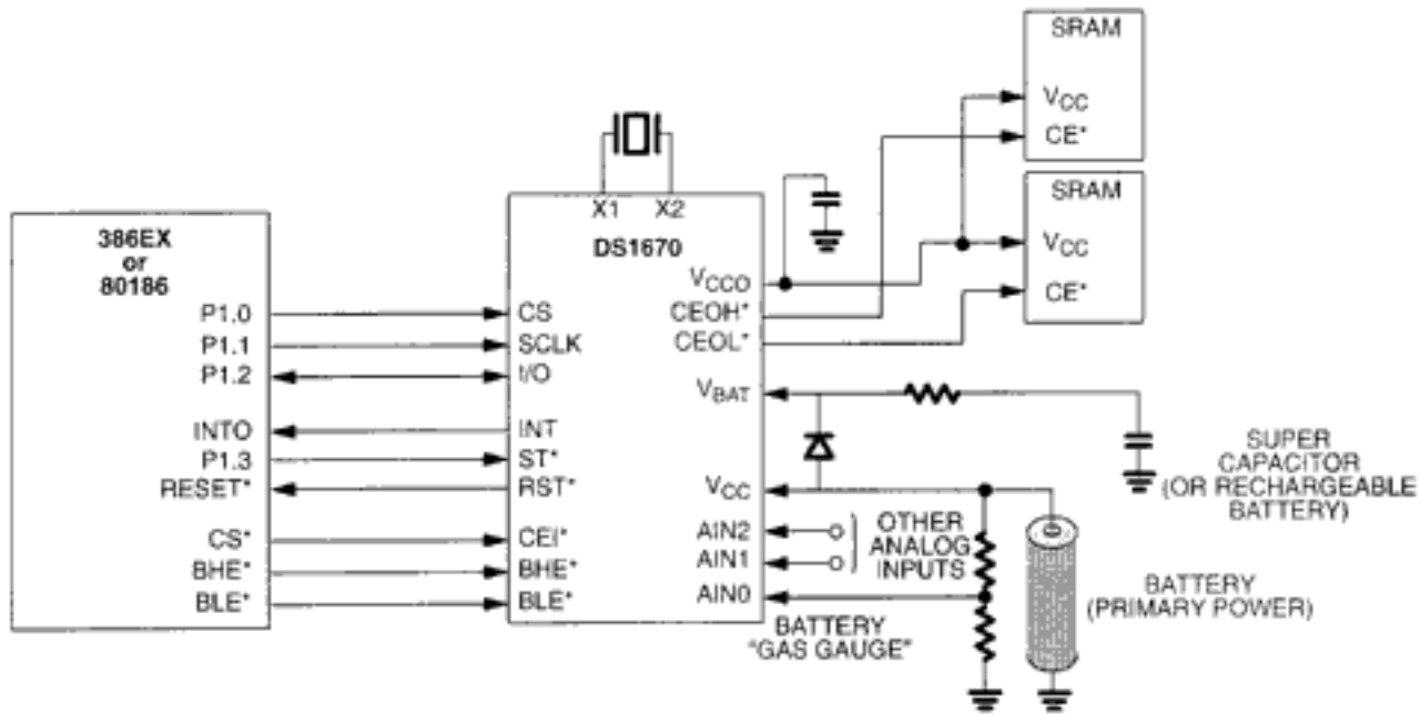
Figure 2. Typical Application
